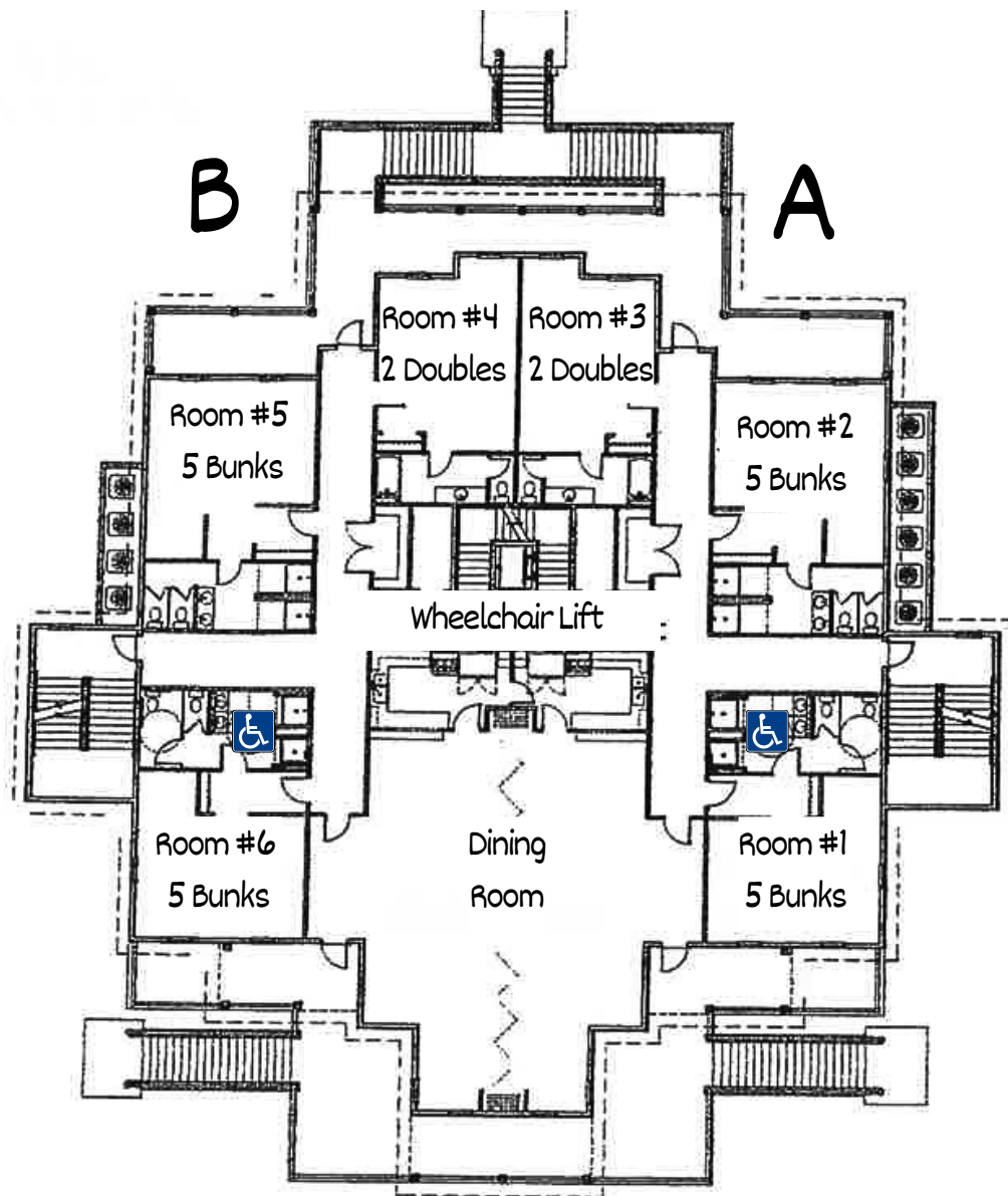
FIRST FLOOR
